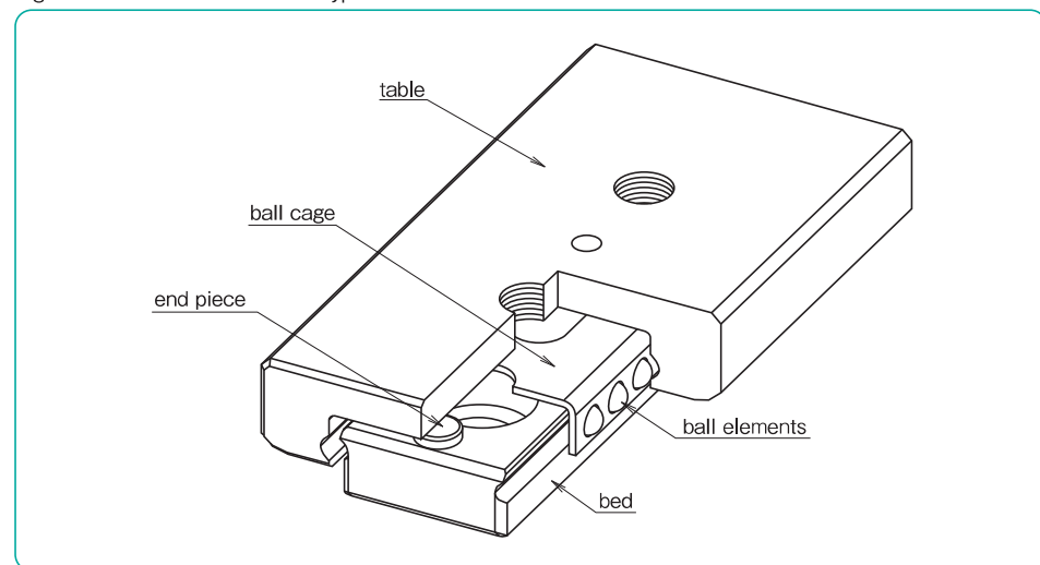
Figure A-24 Structure of SYBS type
