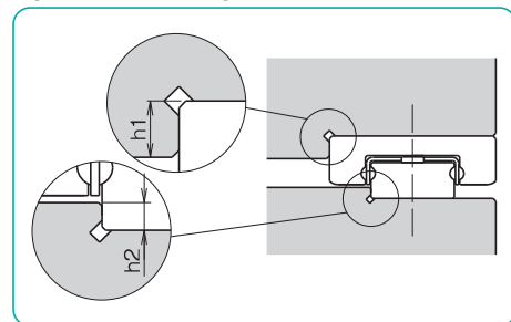
Figure A-28 Mounting Surface Profile-2
