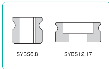
Figure A-29 Profile of SYBS Bed
