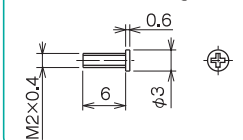
SYBS12 bed mounting screw
