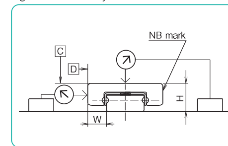
Figure A-25 Accuracy Measurement Method
