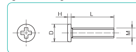
Figure A-31 Mounting Screw
